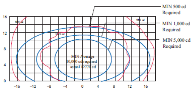
Wingbar, ICAO Fig A2-4, Green
