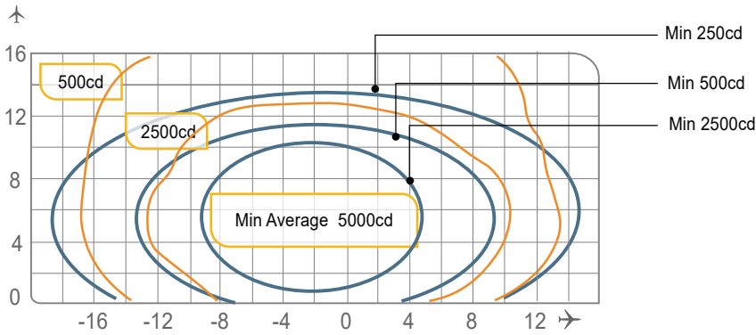
APSS-12-LED, ICAO Fig. A2-2, Red
