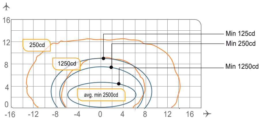
TAES-12-LED, ICAO Fig. A2-8, Red, FAA L-850D
