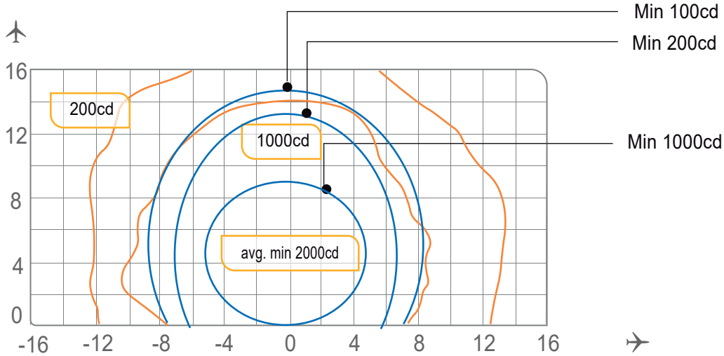
END-12, ICAO Fig. A2-8, Red
