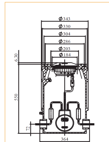
Figure 3 On 12" deep base with 12 7/8" adapter ring
