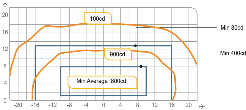
TCLMS-08-S-LED, ICAO Figura A2-12, Green
