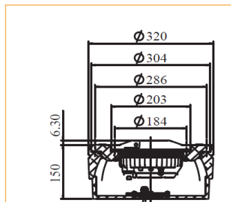
Figure 2 On 12" shallow base with 12 7/8" adapter ring
