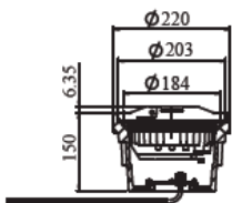
Fig 1. On 8" shallow base
