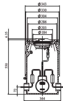
Fig 3. On 12" deep base w/ 12"/8" adapter ring
